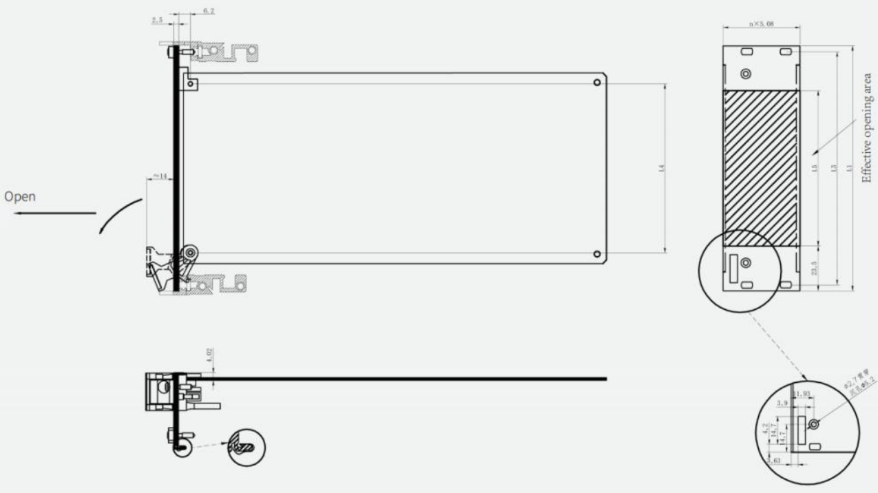
Effective opening area
